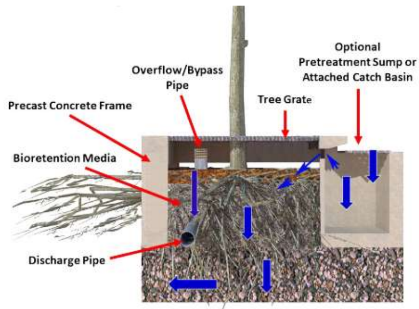
Figure 4: Schematic of tree well configuration
